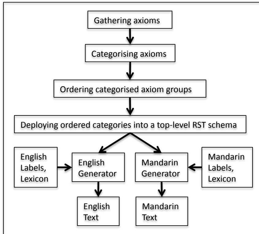
Fig. 1 The system architecture of OntoVerbal-M
