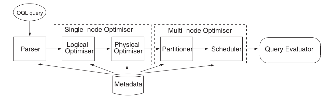
Fig. 3 The components of Polar* query compiler.
