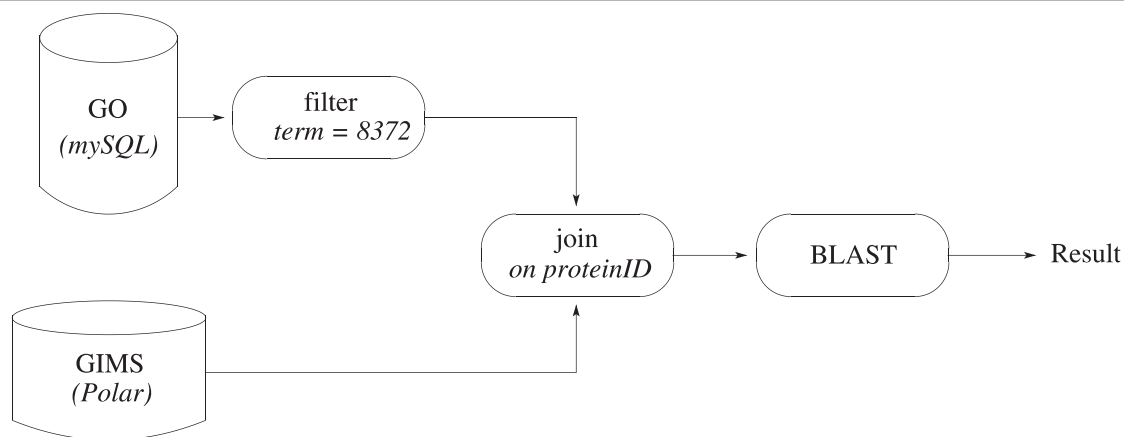
Fig. 1 Evaluating the example query.
