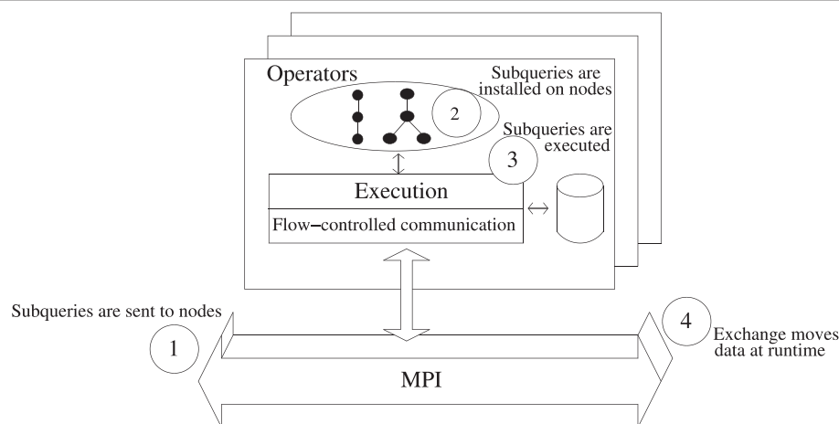
Fig. 6 The different phases involved in planting and executing a query on Grid nodes. Phases 1 and 2 are executed once for each query at the beginning, while phases 3 and 4 are executed concurrently many times.
