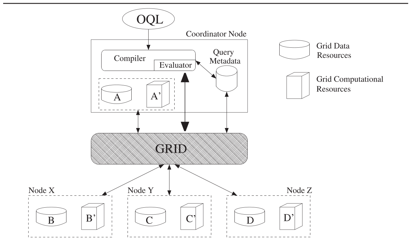
Fig. 2 The Polar* architecture.
