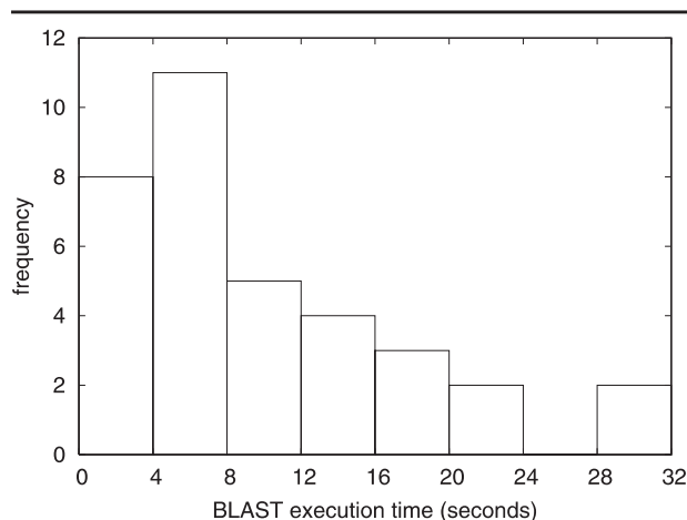
Fig. 9 The variation of the costs of the BLAST calls for the ncl-pc1 .
