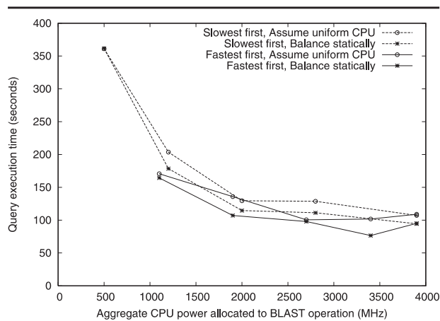
Fig. 10 Measured performance of the example query when the BLAST call is parallelized according to fastest-processor-first and slowest-processor-first .
