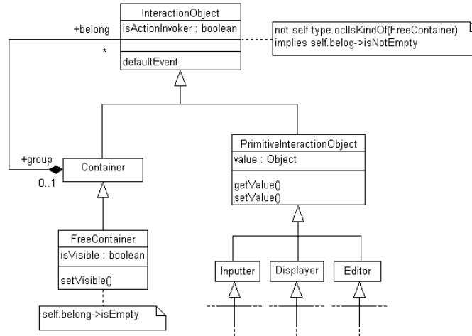
Figure 3: The Abstract Presentation Pattern
