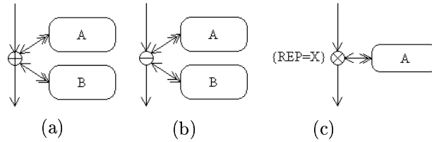
Figure 8: The UMLi modelling of an order independent selection state in (a), an optional selection state in (b), and a repeatable selection state in (c).
