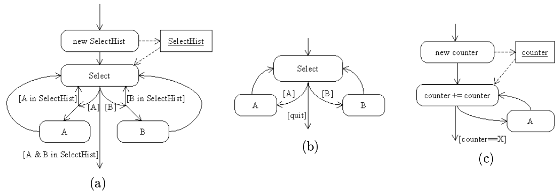
Figure 7: The UML modelling of three common interaction application behaviours. An order independent behaviour is modelled in (a). An optional behaviour is modelled in (b). A repeatable behaviour is modelled in (c).
