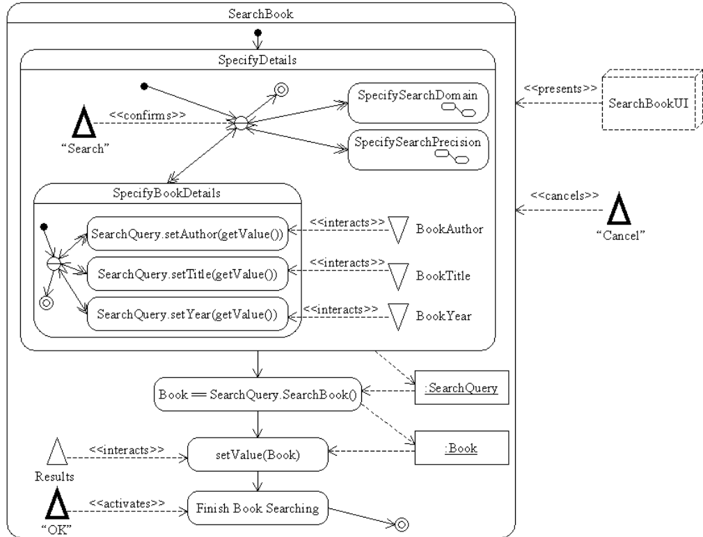
Figure 9: The SearchBook activity.
