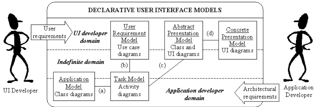
Figure 1: UML i declarative user interface models. The area identified as indefinite domain is where UI developers and application developers may collaborate in terms of a UI design contract elaboration.
