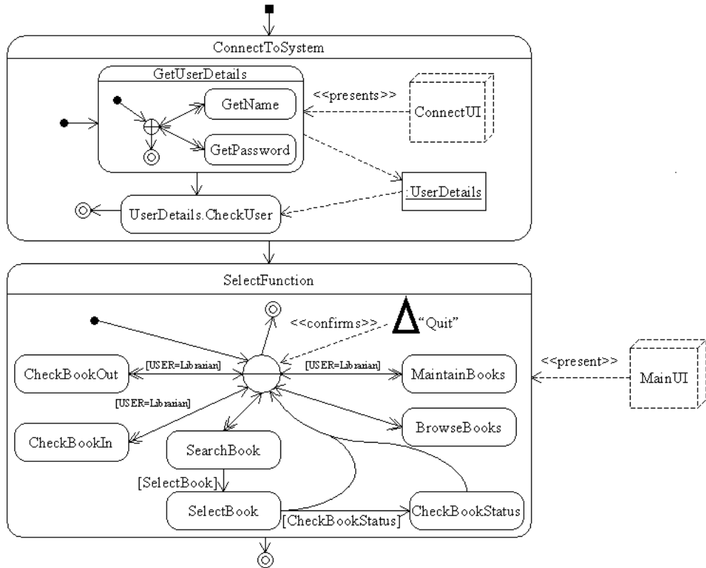
Figure 10: A top interaction activity diagram for the Library case study.
