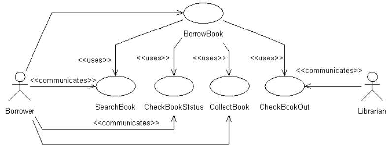
Figure 4: A use case diagram for the BorrowBook use case with its component use cases.
