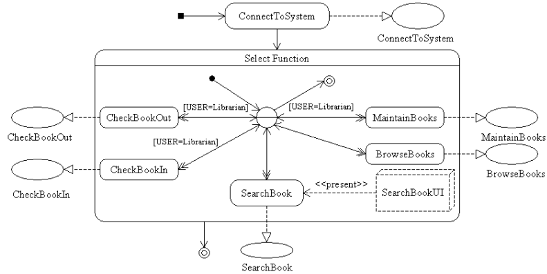
Figure 6: Modelling an activity diagram from use cases using UMLi.
