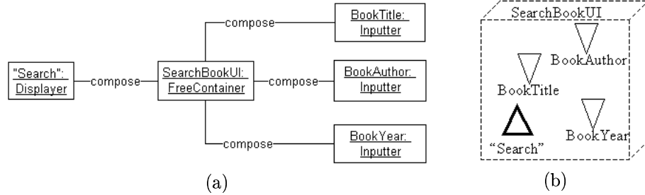
Figure 2: An abstract presentation model for the SearchBookUI can be modelled as an object diagram of UML, as presented in (a). The same presentation can alternatively be modelled using the UMLi user interface diagram , as presented in (b).
