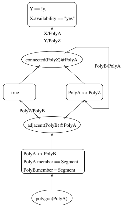
Fig. 8: Example system graph for ROLL rule.
