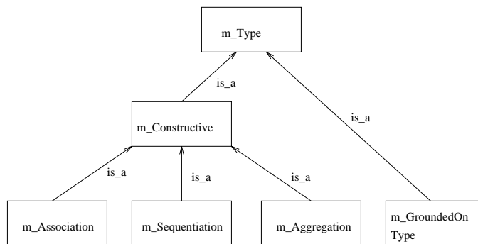
Fig. 4: E classes for describing OM types
