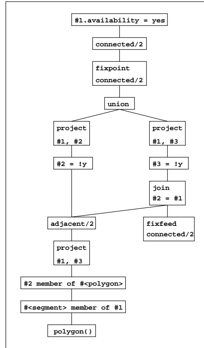
Fig. 11: Example processing tree after global optimization
