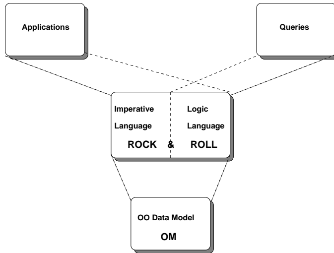
Fig. 1: Relationship between the principal components in the architecture.
