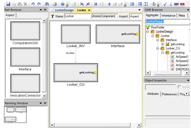
Fig. 7. Component Designer: Component life cycle.
