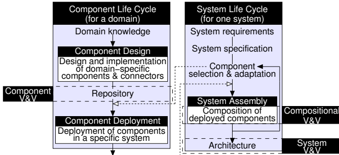
Fig. 5. X-MAN CBD process with V&V.
