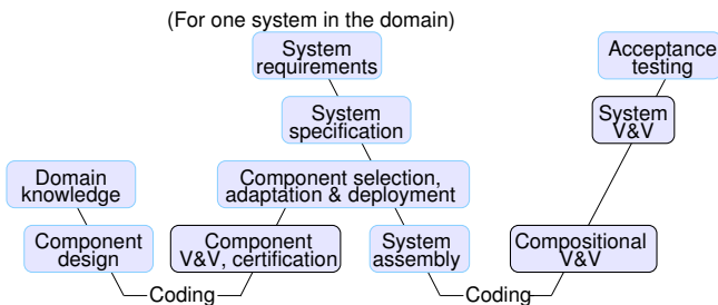
Fig. 6. The W Model.
