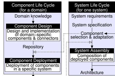
Fig. 4. X-MAN CBD process.
