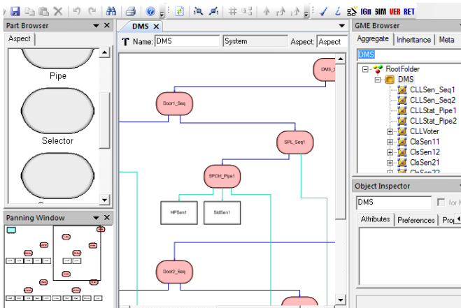
Fig. 8. System Assembler: System life cycle.
