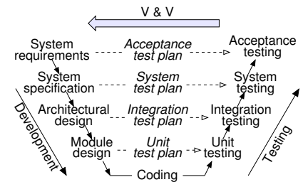
Fig. 2. The V Model.
