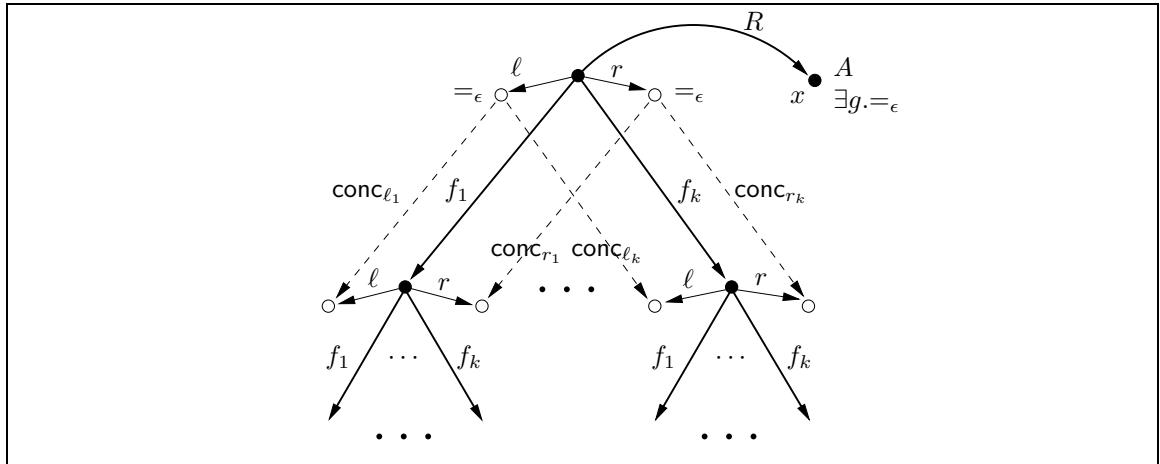
Figure 2: An example model of C_P and \mathcal{K}_P .
