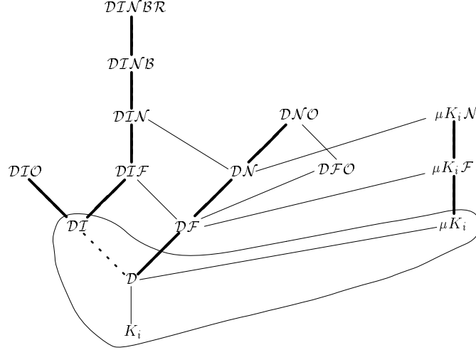
Figure 1.2: Propositional dynamic logics studied in the thesis
