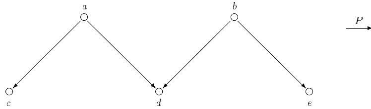
Figure 4.1: A model of a \mathcal{DIF} formula \Phi
