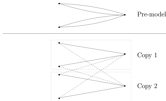
Fig. 4. The copying construction.
