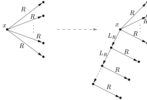
Fig. 5. Representing role neighbour relationships.
