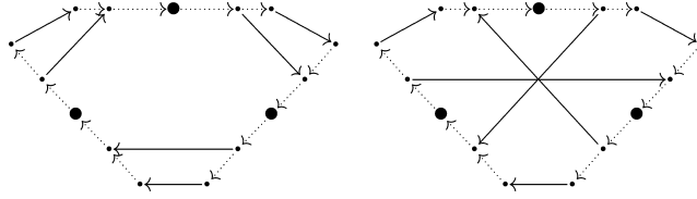
Fig. 7. Two models for \sigma(C) and \sigma(T) .
