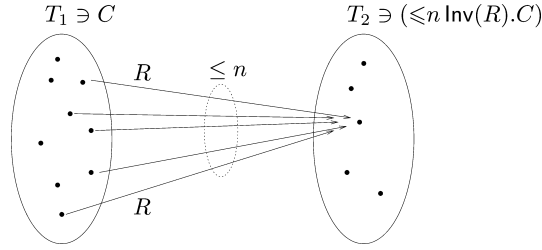
Fig. 3. Illustration of the lim function.
