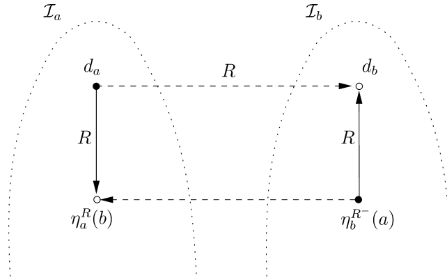
Fig. 8. Connection of the models \mathcal{I}_a and \mathcal{I}_b .
