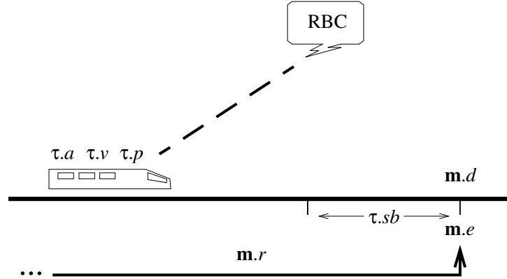
Figure 15: The European Train Control System. A generalised movement authority, defined by its recommended speed limit m.r , end position m.e and demanded speed limit (at end) m.d . This is used to control the train parameters: train acceleration \tau.a , train speed \tau.v , and train position \tau.p . The essential safety invariant is \tau.p \geq m.e \Rightarrow \tau.v \leq m.d .
