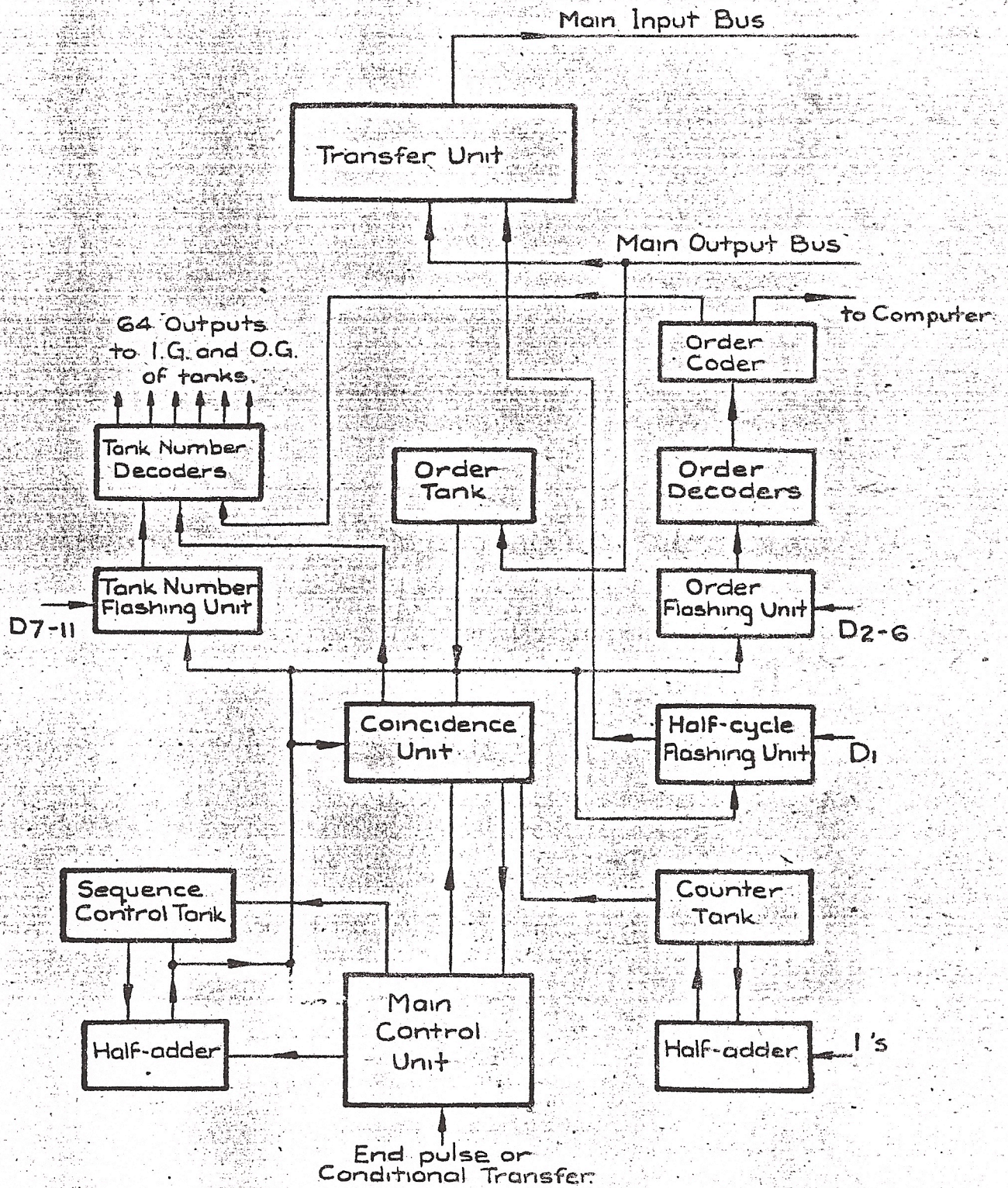
Fig.3. MAIN CONTROL UNIT. Schematic.
