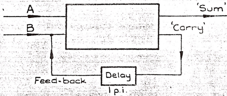
Fig. 4(a) HALF-ADDER
