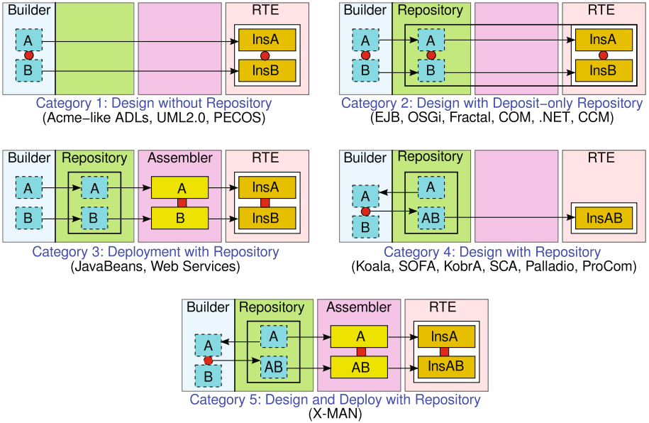
Fig. 5. Idealised component life cycle: taxonomy of component models.
